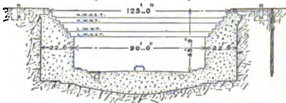
FIG. 27.—Cross Section of Southampton Graving Dock.
