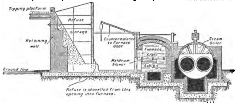
FIG. 3.—Meldrum's Destructor at Darwin.
