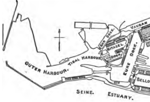
FIG. 2.—Havre Docks and Outer Harbour.
