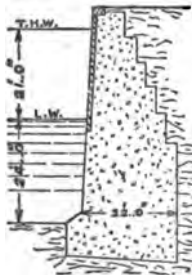
FIG. 11.—Tilbury Basin Wall.
