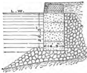
FIG. 13.—Marseilles Quay Wall.
