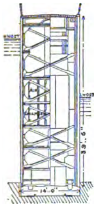
FIG. 24.—Sliding Caisson.
