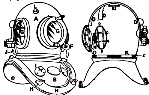
Front view of Helmet.
