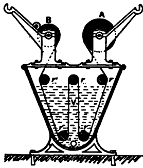
FIG. 3.—Dye-jigger.
