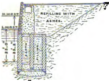
FIG. 16.—Glasgow River Quay Wall.
