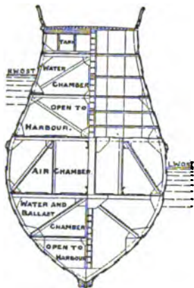
FIG. 25.—Ship Caisson.
