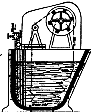
FIG. 4.—Dye-vat for Piece Goods.
