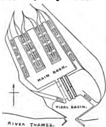
FIG. 7.—Tilbury Docks
