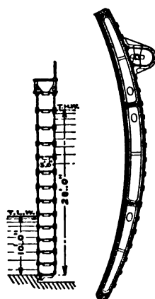
FIG. 22.—Iron Segmental Dock Gate.
