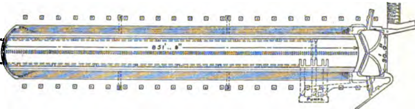
FIG. 26.—Plan of Southampton Graving Dock.
